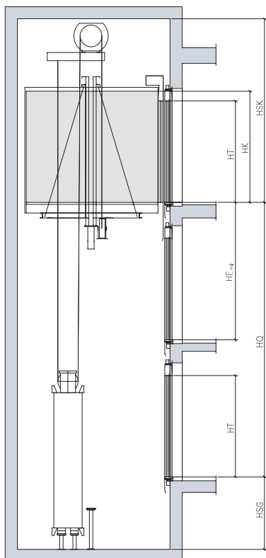
One-sided entrance
